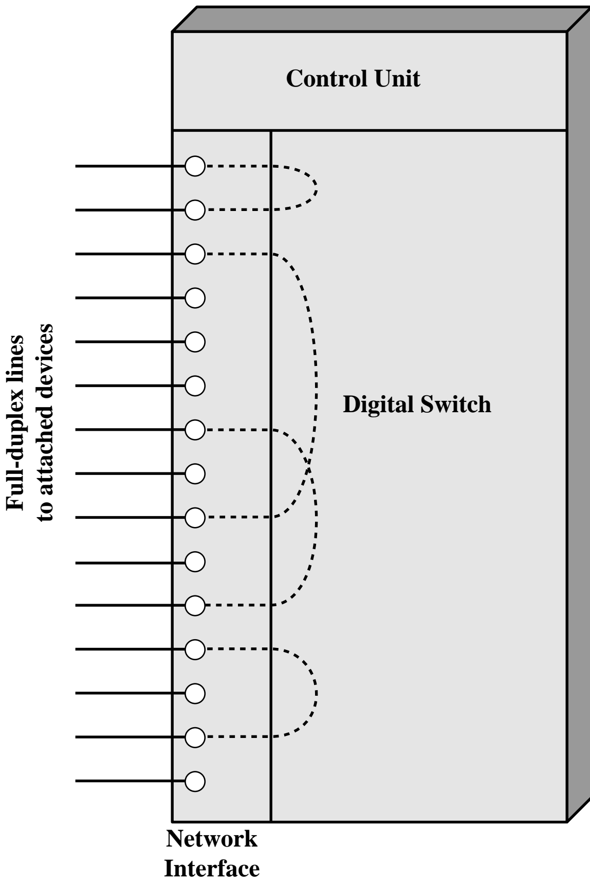
Figure 7.5 Elements of a Circuit-Switch Node
