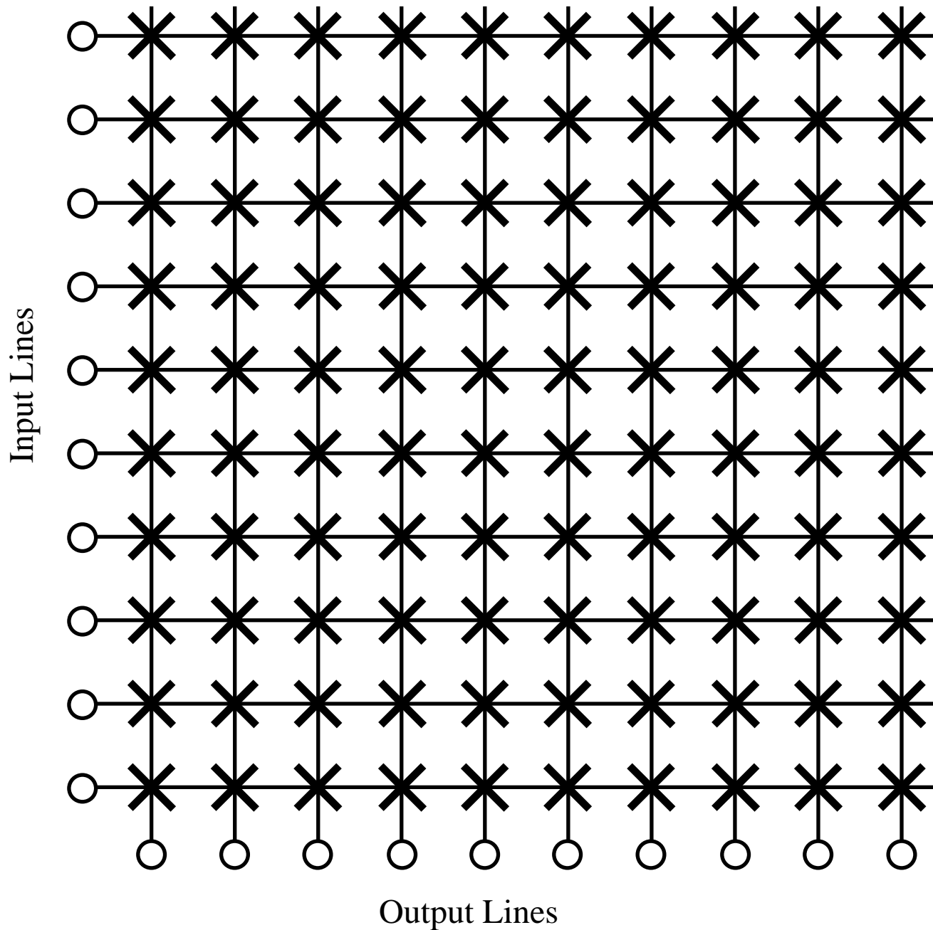
Figure 7.6 Space-Division Switch
