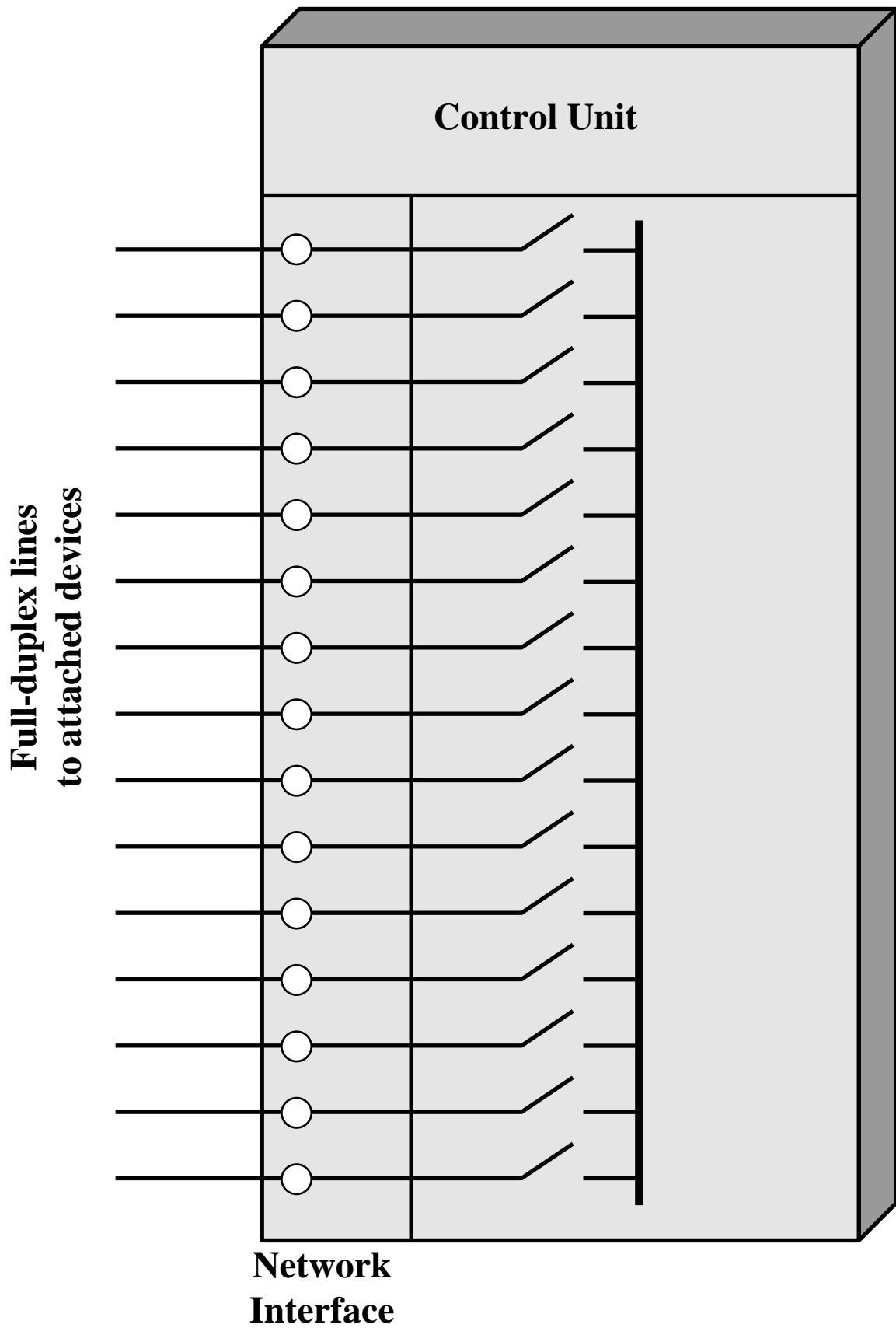
Figure 7.7 TDM Bus Switching
